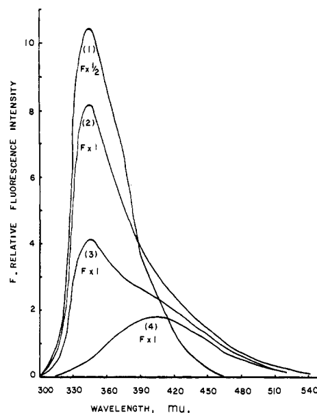
Figure 1. Concentration dependence of monomer and excimer fluorescence of acetone in n -hexane solutions at 25° ( \lambda_{\text{exo}} 285 m\mu ): (1) 2.7 \times 10^{-4} M , (2) 2.7 \times 10^{-3} M , (3) 1.1 \times 10^{-2} M , (4) 2.2 \times 10^{-2} M .
